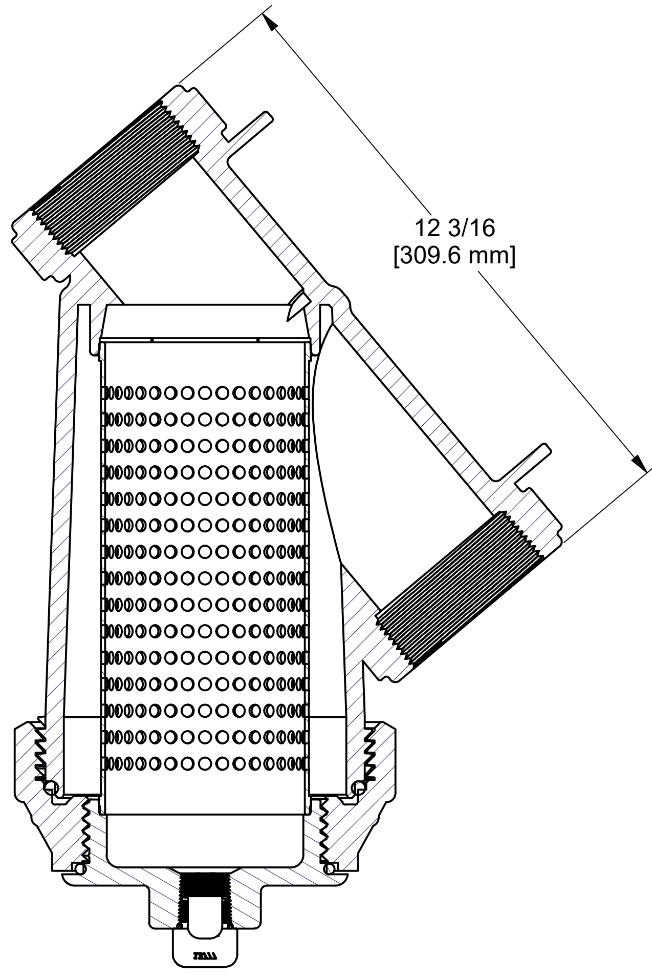
SECTION B-B SCALE 1:2
